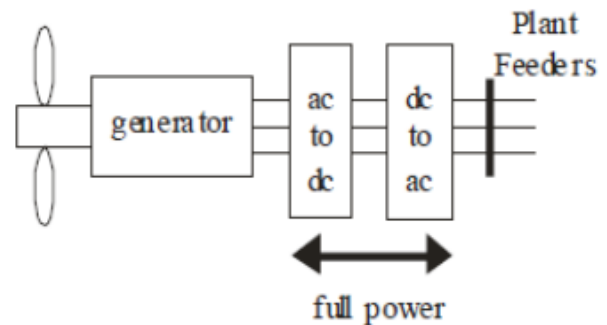
Fig 5: wind turbine generator assembly
