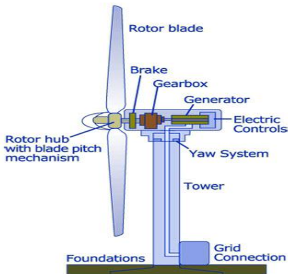
Fig 4: Wind turbine system
