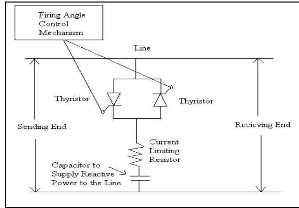
Fig 2: pf improvement using TSC
