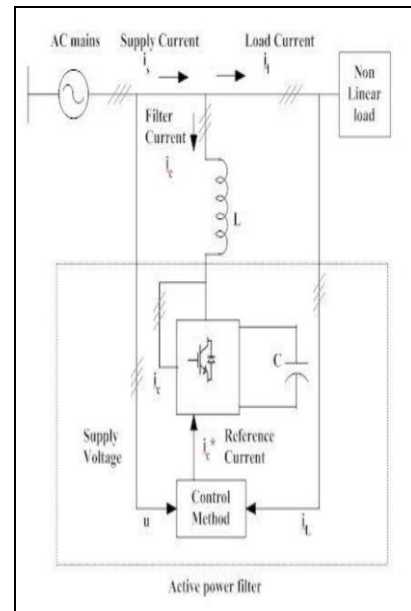
Fig 4: Schematic diagram of shunt connected active power filter
