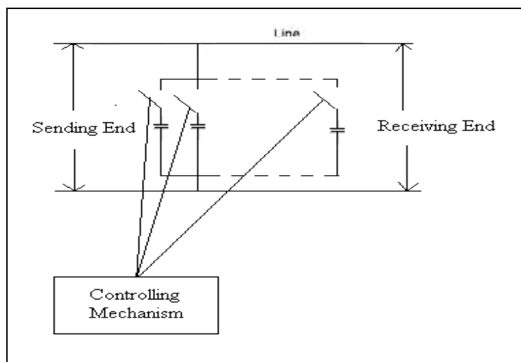
Fig 1: pf improvement using capacitor bank
