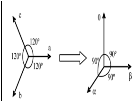
Fig 5: Transformation from the phase reference system (ab c) to the (0αβ) system [5].
