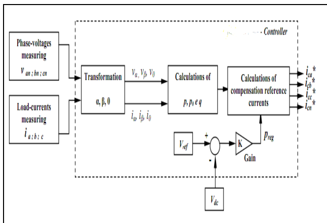
Fig 6: Calculations of the p-q theory
