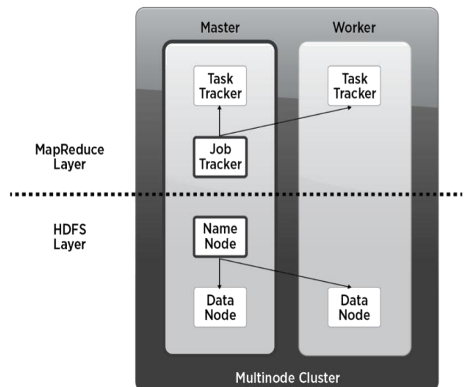
Fig 1: A simplified overview of Hadoop
