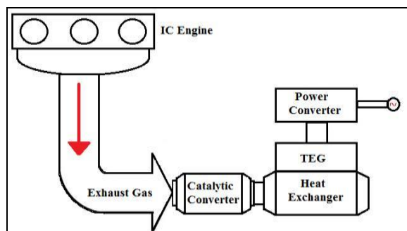
Fig 2: Thermoelectric Generator
