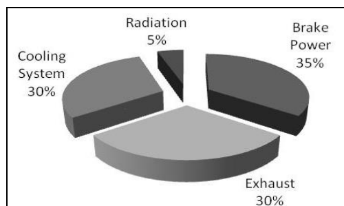
Fig 1: Total fuel energy content in I. C. engine
