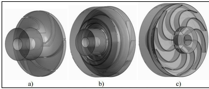
Fig 1: Three dimensional calculation domain, a) Entrance duct and impeller, b) Front view of pump, c) Back view of pump
