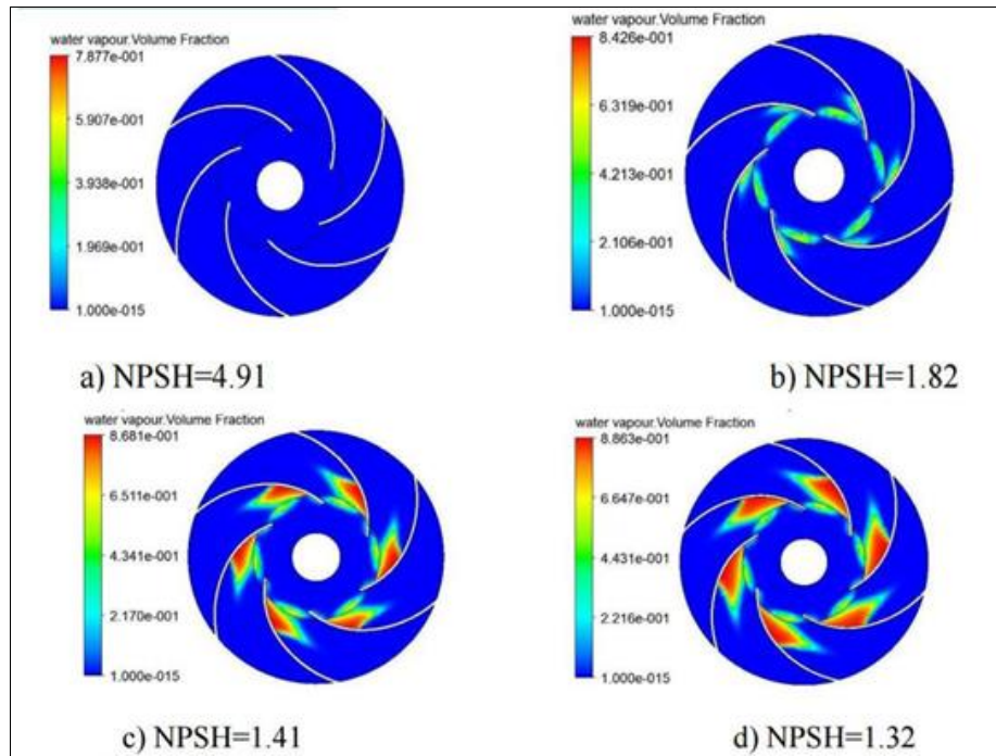
Fig 3: Vapor phase distribution in the front view of impeller in difference NPSH
