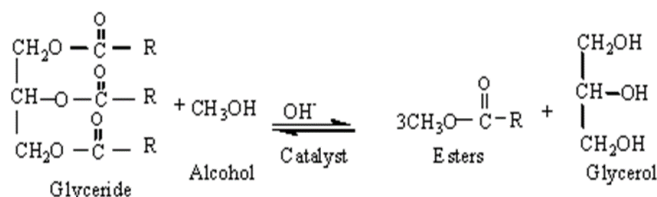
Fig 1: Transesterification Process
